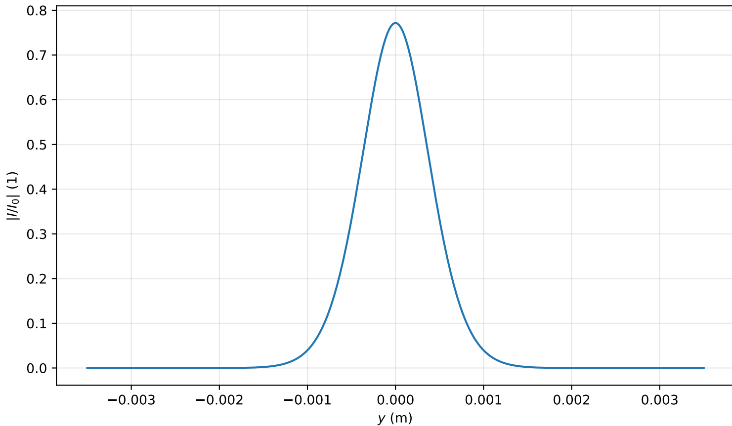
Intensity profile I(x=0, y, z=1.592)/I_0 , P_{in}=0.3P_{cr} , artificial time
